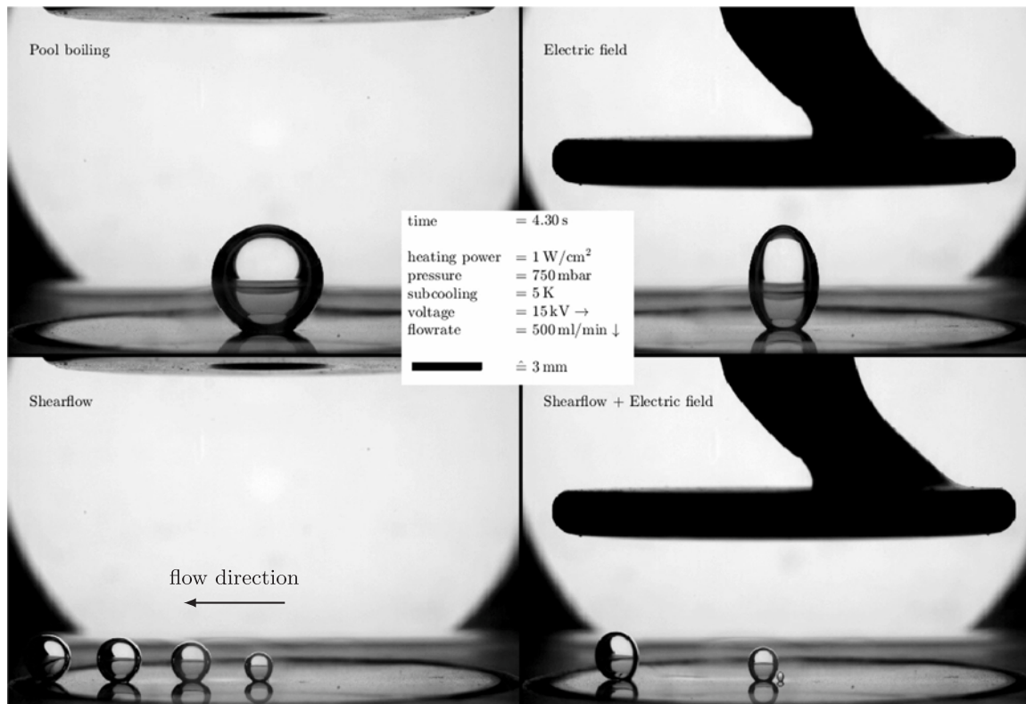
Fig. 12. Comparison of the different external forcing factors.
